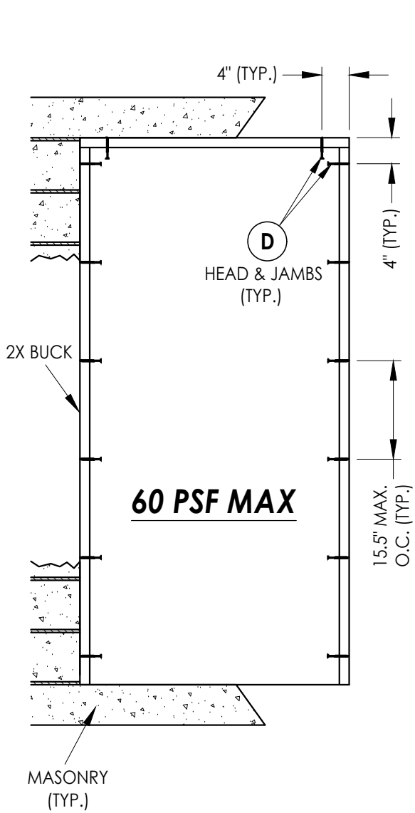
2X BUCK ANCHORING
