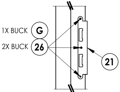
MULTIPOINT LATCH & DEADBOLT STRIKE DETAIL
